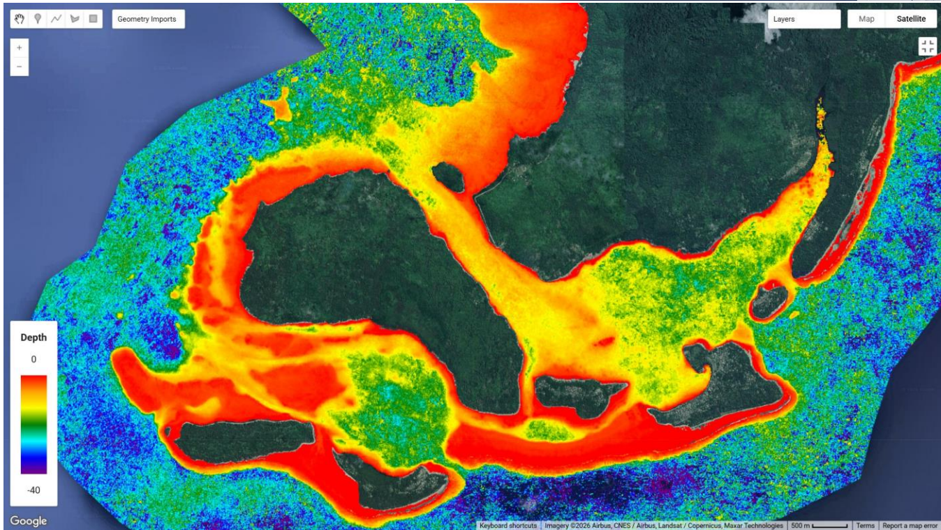
10m -Satellite Derived Bathymetry (Sentinel-2)
