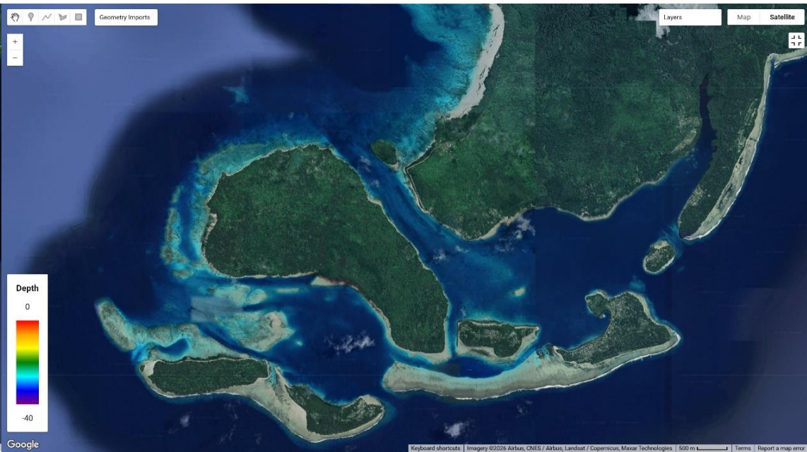
10m -Satellite Derived Bathymetry (Sentinel-2)
